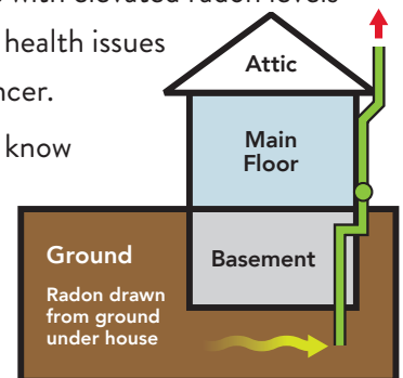
Example of radon mitigation system
